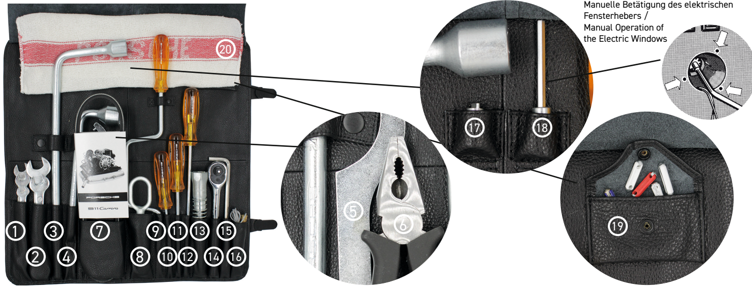
Radwechsel / Changing Road Wheel
